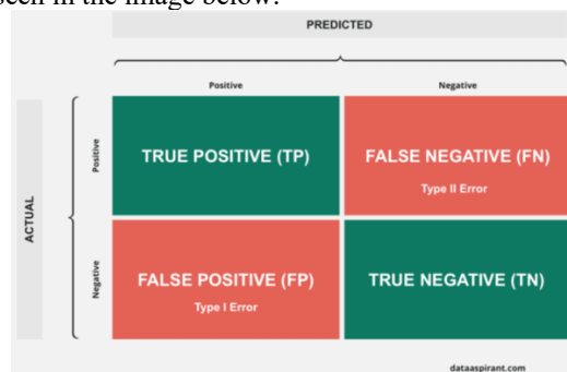
Figure 2. Confusion Matrix
